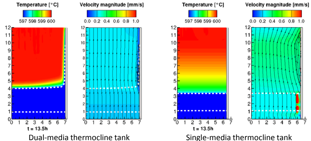
Dual-media thermocline tank
