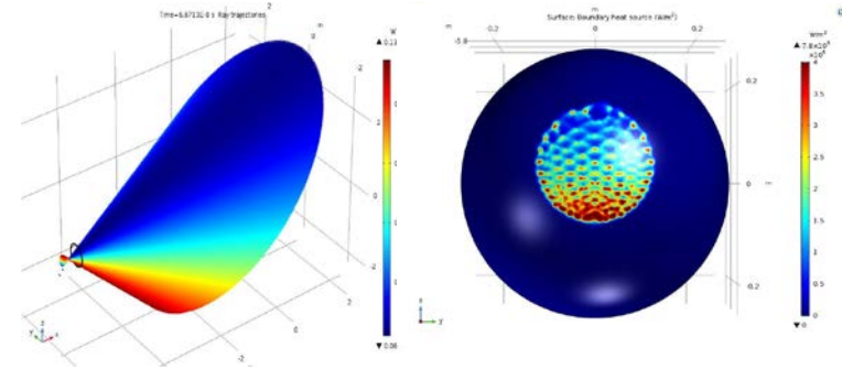
Ray-tracing analysis of the receiver.
